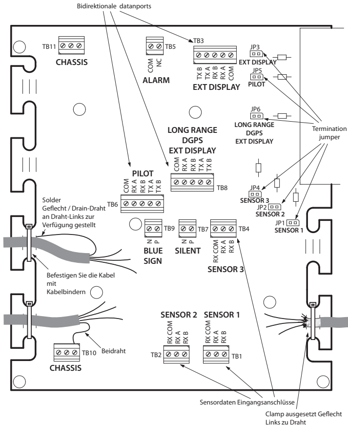
Abbildung 34 Junction-Box-Anschlüsse
